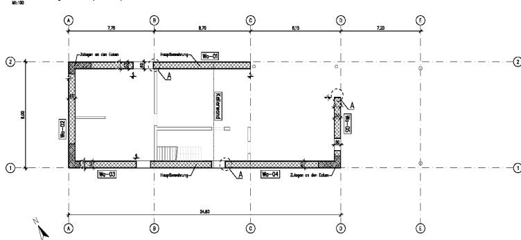
Grundriss Erdgeschoss (+1.00m)
