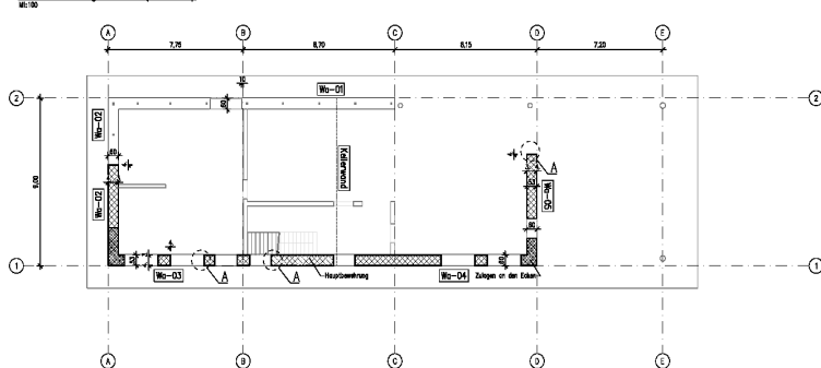
Grundriss Erdgeschoss (+2.90m)
